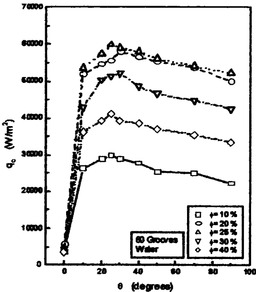
Fig. 11 Plot of heat flux against inclination angle
