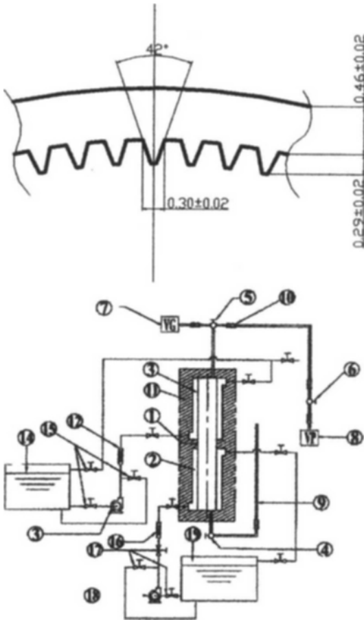
1. Test Tube 2. Heating Water Chamber 3. Cooling Water Chamber 4. Vacuum Valve 5. Vacuum Valve 6. Vacuum Rubber Hose 7. Vacuum Gauge 8. Vacuum Pump 9. Measuring Device for Liquid 10. Vacuum Rubber Hose 11. Insulation 12. Coolant Flow Meter 13. Coolant Pump 14. Coolant Constant Temperature Bath 15. Coolant Control Valve 16. Heating Water Flow Meter 17. Heating Water Control Valve 18. Heating Water Pump 19. Heating Water Constant Temperature Bath
