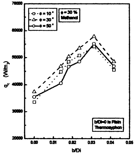
Fig. 15 Effects of the distance between grooves on the measured average heat flux
