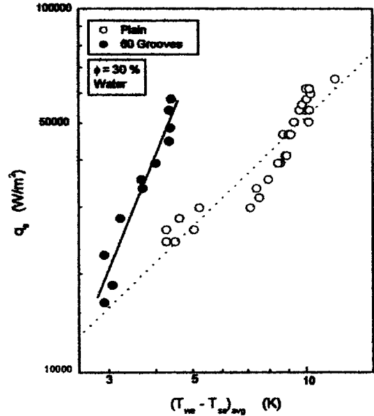
Fig. 6 Measured average heat flux vs. temperature excess (The solid and dotted line were determined by a least squares method.)
